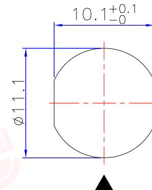
PANEL CUTOUT
