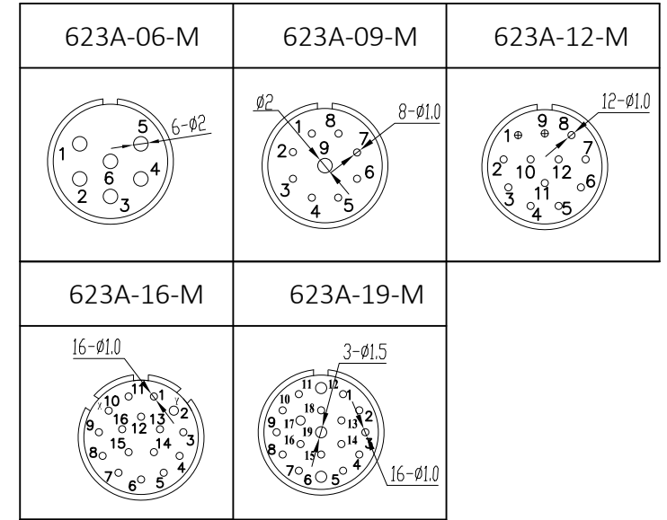
Pin Assignment (View A)
